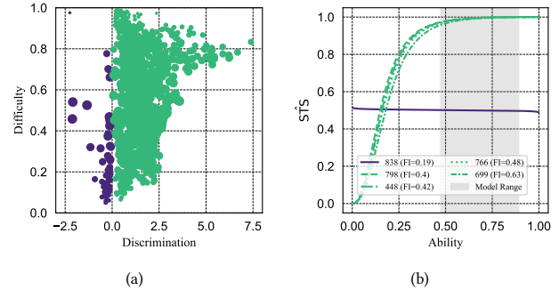
Figure 6: The plots for the Adult dataset with race the sensitive attribute: (a) The scatter plot shows the discrimination parameter a j and the difficulty parameter δ j for each individual; (b) Examples of selected individuals with flat ICCs. The shaded area indicates the ability range of the 14 selected predictive models.
