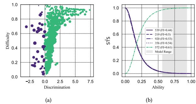
Figure 5: The plots for the Law School dataset: (a) The scatter plot shows the discrimination parameter a_j and the difficulty parameter \delta_j for each individual; (b) Examples of selected individuals with flat ICCs. The shaded area indicates the ability range of the 15 selected predictive models.
