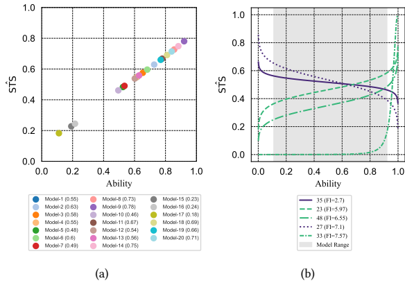
Figure 3: (a) The scatter plot shows the \hat{S}T\hat{S}_i and ability parameter \theta_i for each predictive model; (b) Examples of selected individuals with flat ICCs. The shaded area indicates the ability range of the 20 selected predictive models.
