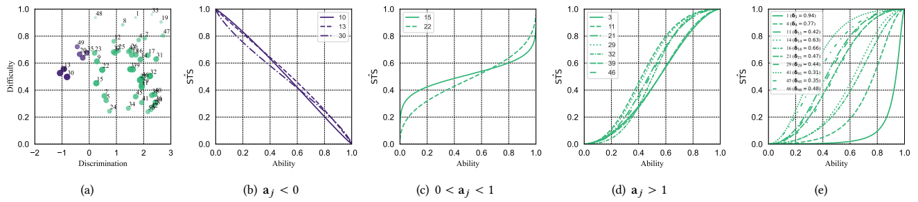
Figure 2: (a) The scatter plot shows the discrimination parameter a_j and difficulty parameter \delta_j for each individual. The purple points indicate individuals with negative discrimination values (special individuals), while the green points indicate individuals with positive discrimination values (normal individuals). The size of the points increases as \delta_j approaches 0.5 and gradually decreases as \delta_j approaches 0 or 1; (b,c,d) Examples of ICCs generated by Fair-IRT for different values of discrimination and fixed range of difficulty (i.e., 0.4 < \delta_j < 0.6 ). Higher discriminations lead to steeper ICCs; (e) Examples of selected ICCs for different values of difficulty and fixed range of discrimination (i.e., 1.7 < a_j < 2 ).
